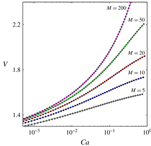
FIGURE 10. (Colour online) Influence of the viscosity contrast, M = \mu_w / \mu_g , on the speed of the Type I travelling waves, as a function of capillary number, Ca . We set \beta = 8 . This plot elucidates the structure of the constant flux displacements obtained by solving the PDE (figure 3). For a given capillary number, the speed of the plateau increases with viscosity contrast. In terms of displacement pattern, this corresponds to lower plateau heights.
